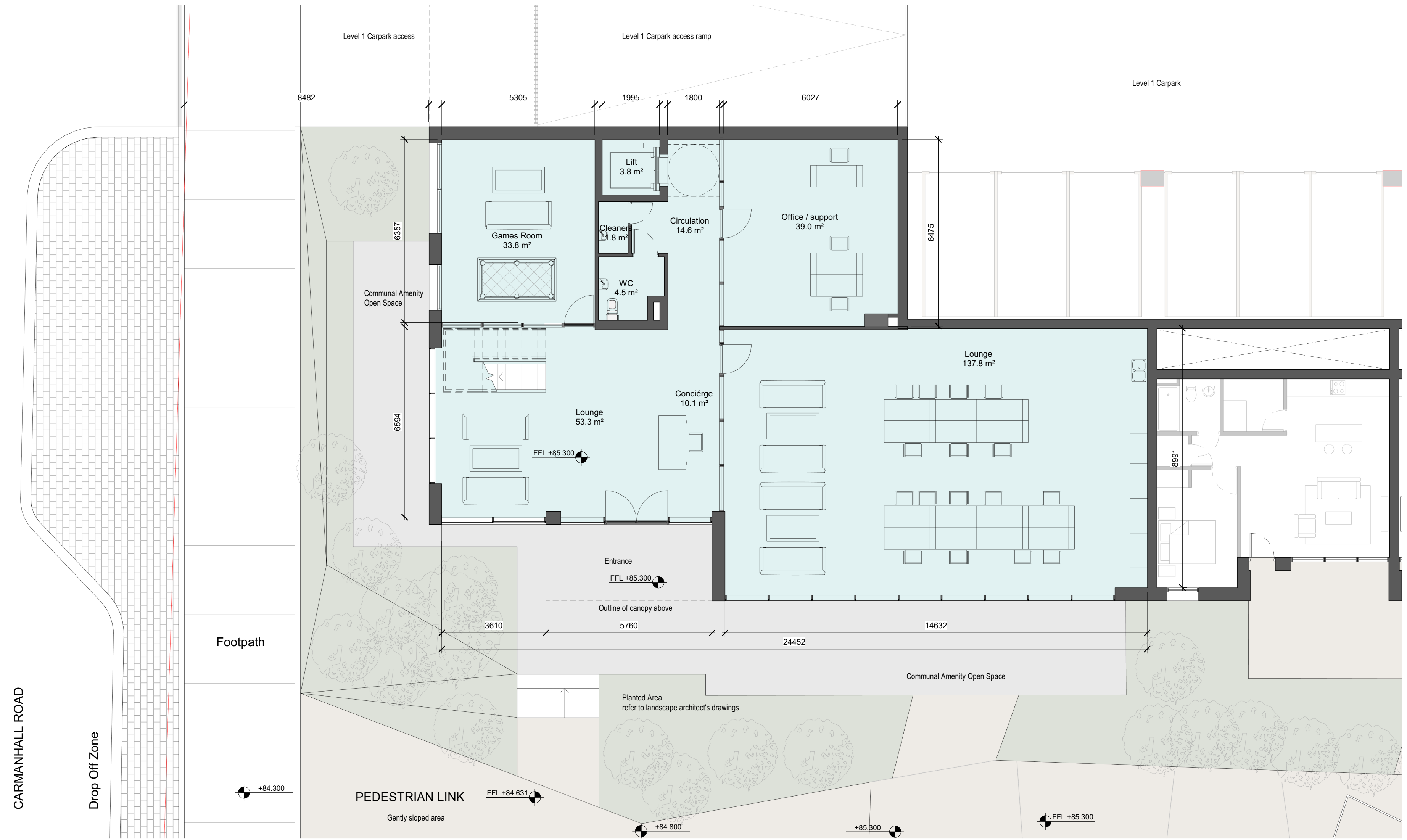
1 Block A Amenities Level 1 (Boulevard Level) 1:100
