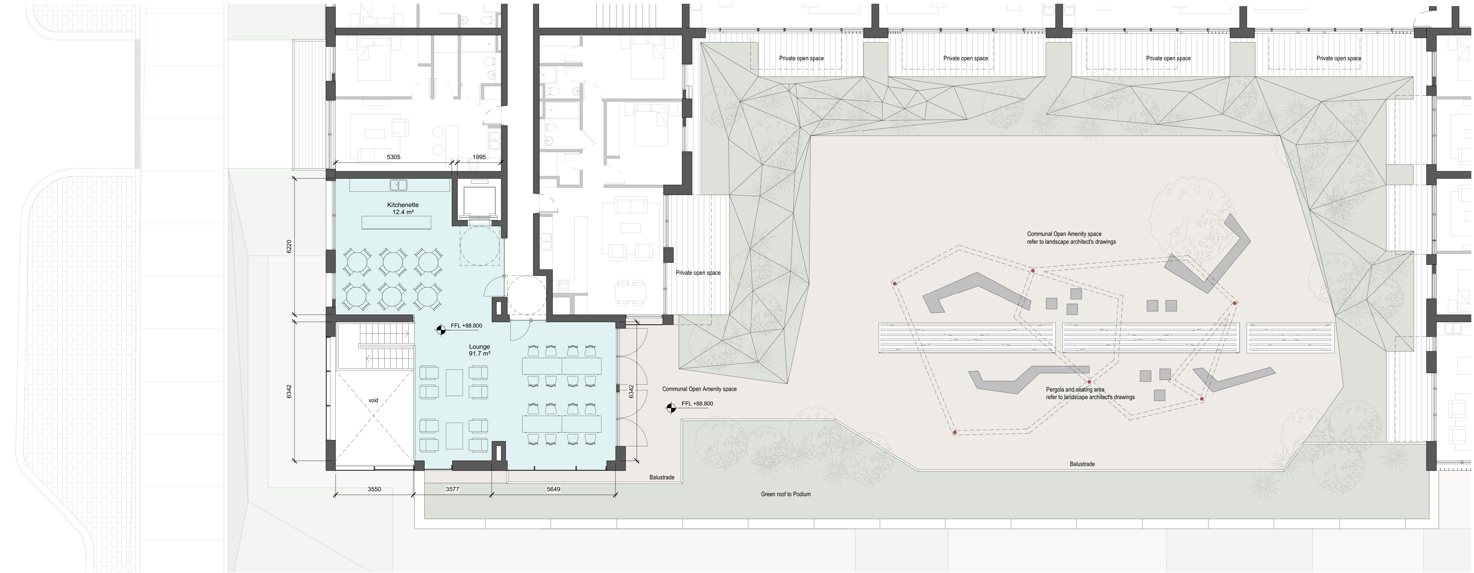
2 Block A Amenities Level 2 1:100
